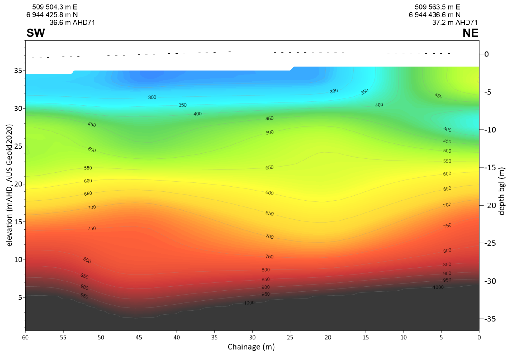
Seismic Line MASW AU-GP 118
